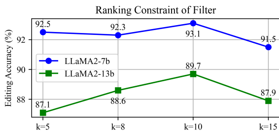
Figure 7: Ablation study results of the ranking constraint k of filter.
