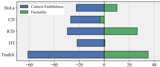
Figure 3: Changes (%) in Context-Faithfulness and Factualty of Factualty-Enhanced LLMs.
