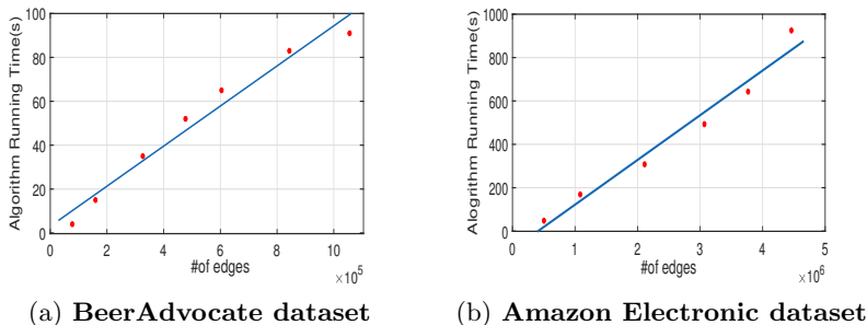
Fig. 4. EigenPulse runs in near-linear time.
